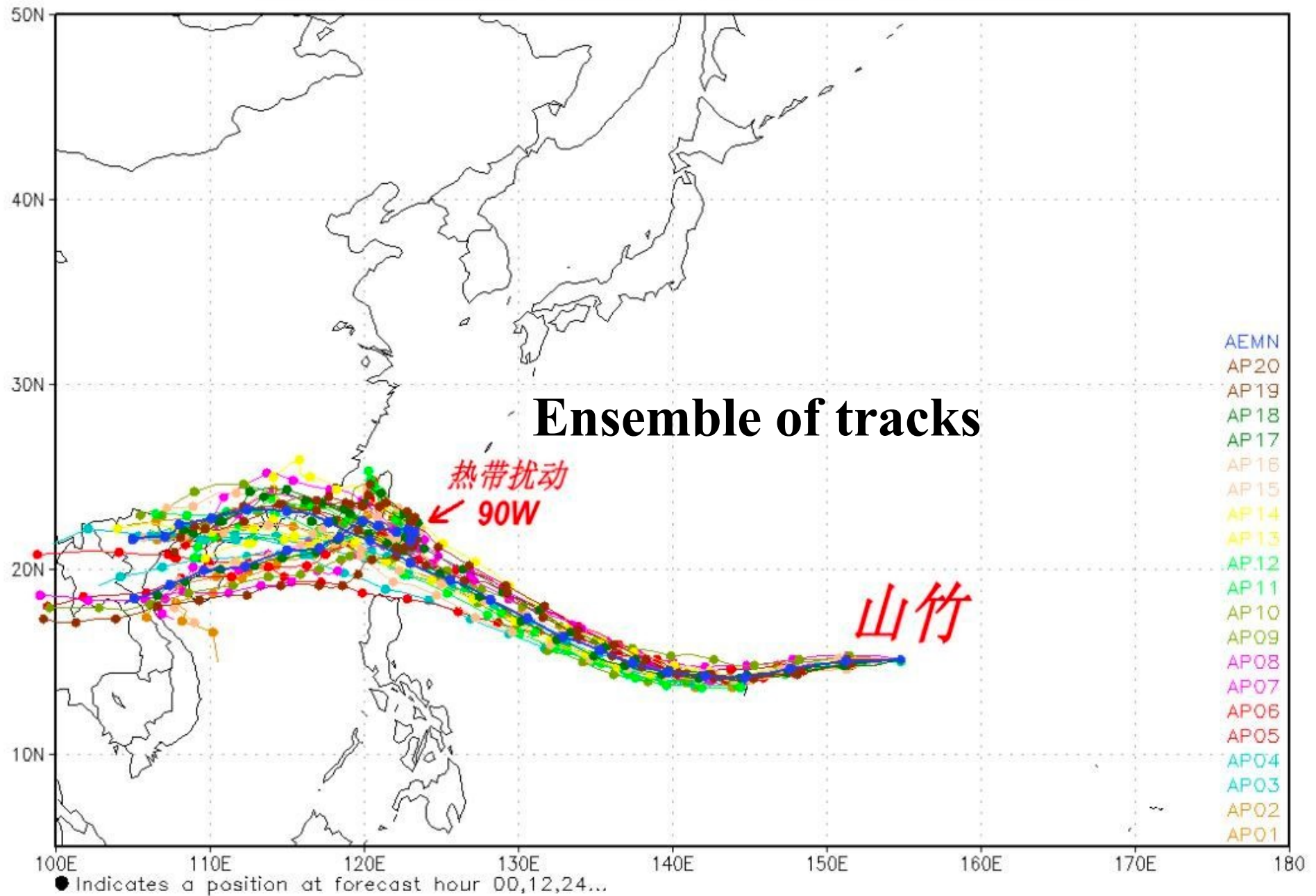
NCEP Ensemble Forecast TC Tracks 2018090900
